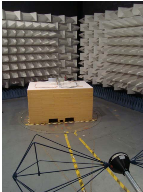
Figure 1 EUT / test set up - spurious radiated emissions ( 30 \text{ MHz} < f < 200 \text{ MHz} )
