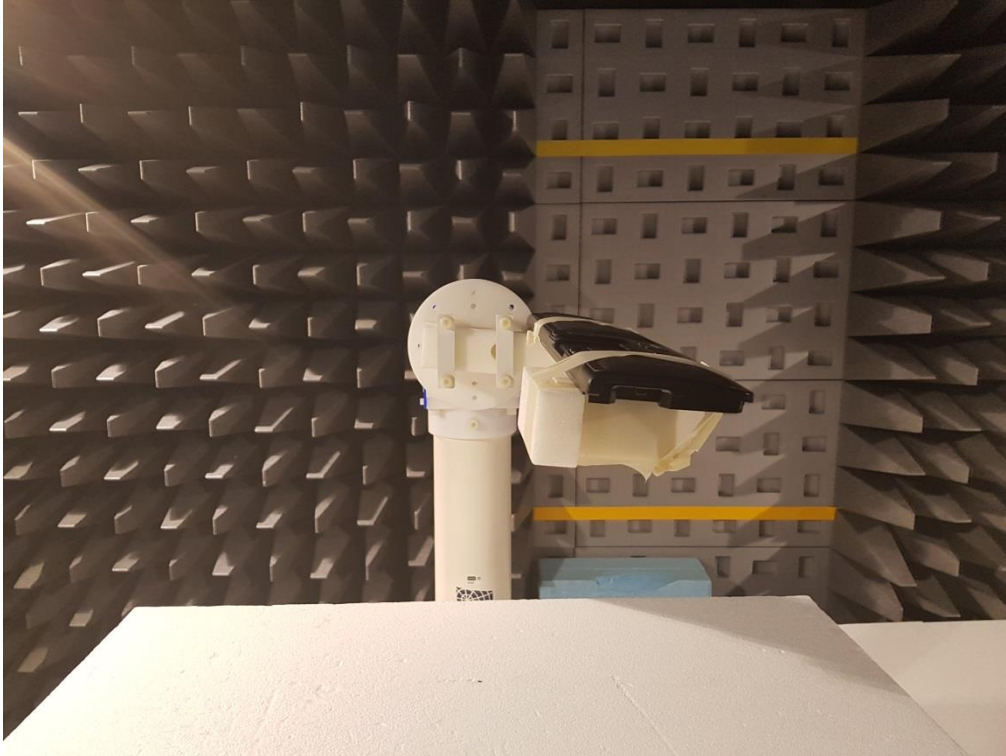
Test set up radiated emission 1GHz – 26.5 GHz
