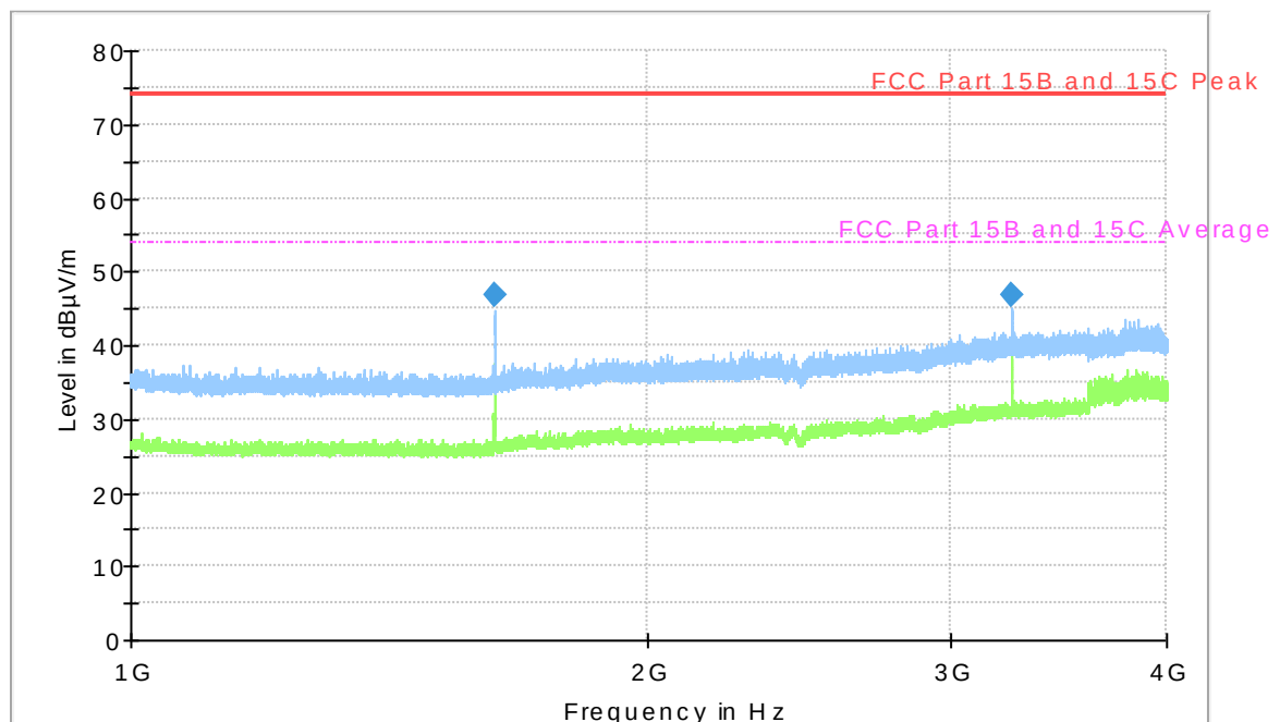
Diagram, Peak overview sweep, 1– 4 GHz at 3 m distance. TX middle channel, Carrier is attenuated by band rejection filter K&L 6N45-2450/T 100-0/0.
