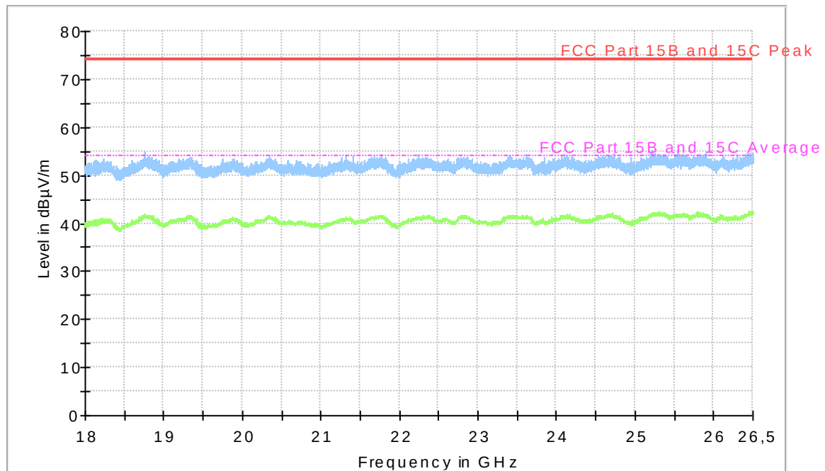
Full Spectrum
