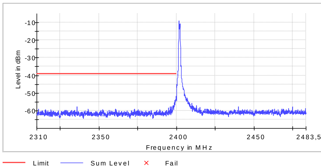
Screenshot: Lower band edge sweep, single channel
