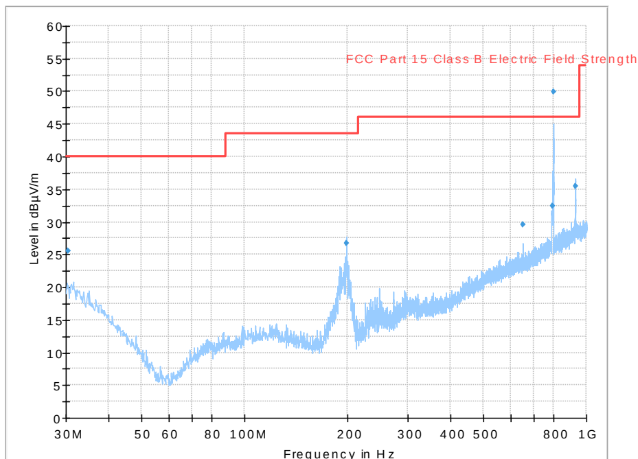
Full Spectrum
