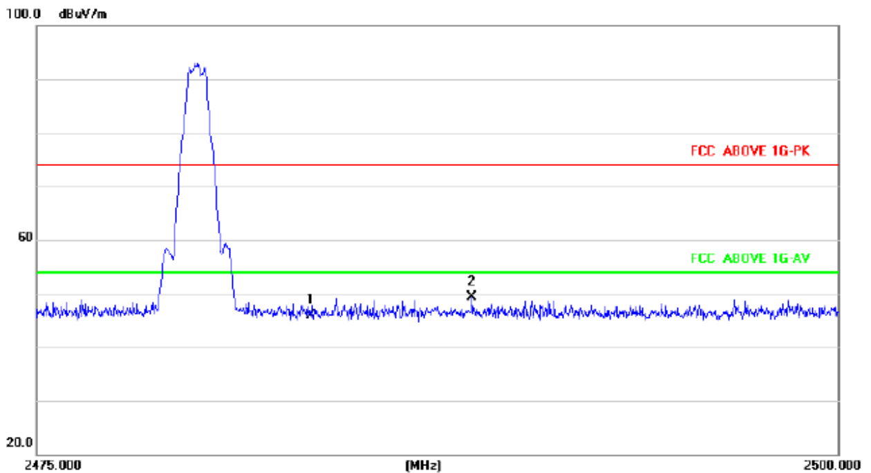
2480MHz Vertical
