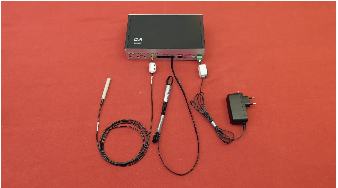
Picture 13: Configuration for radiated tests
