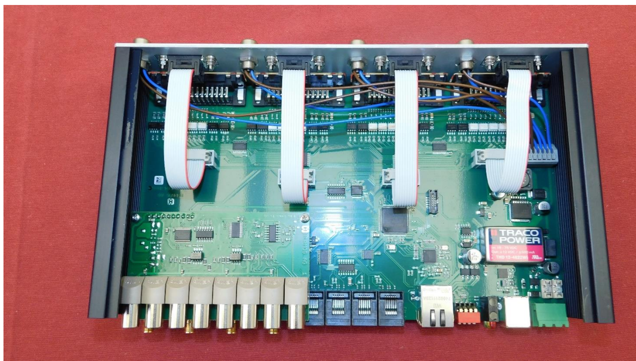
Picture 1: Opened EUT - top side with housing
