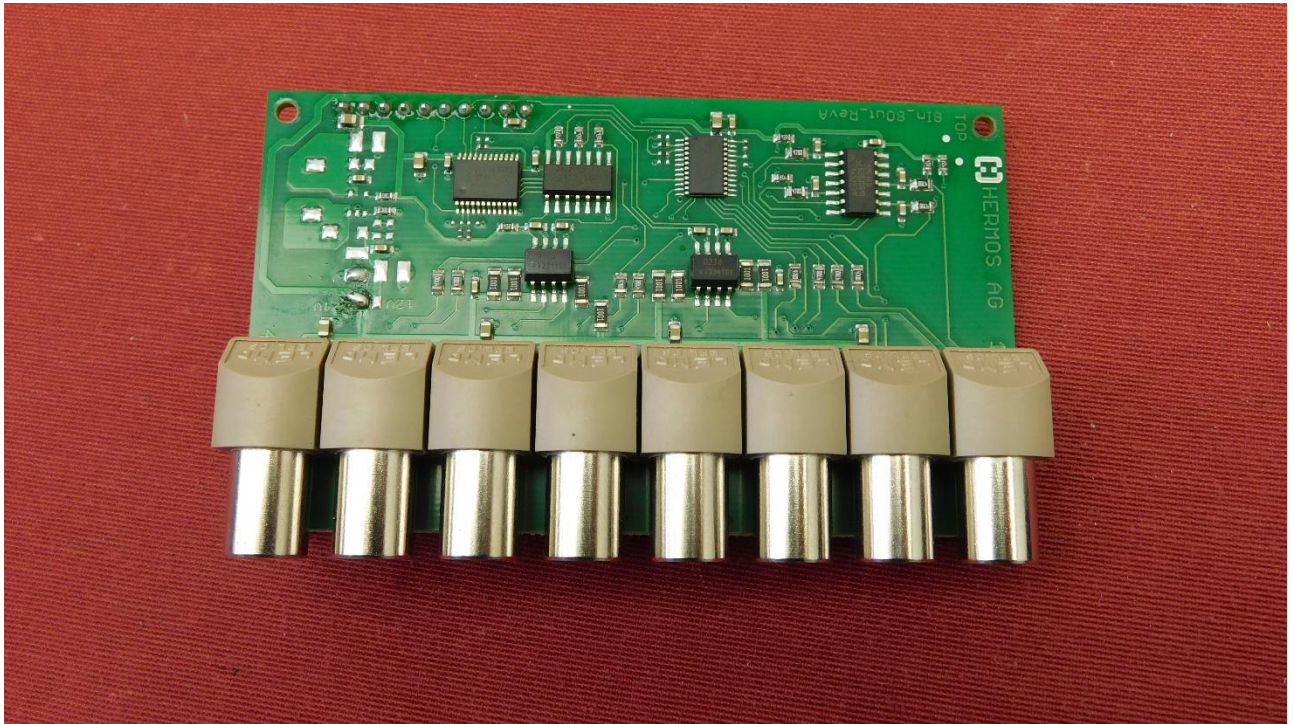
Picture 3: Top view of Input / Output Module
