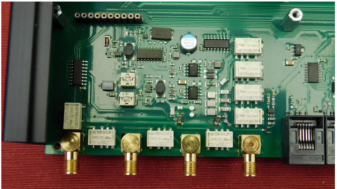
Picture 5: Top view of radio part
