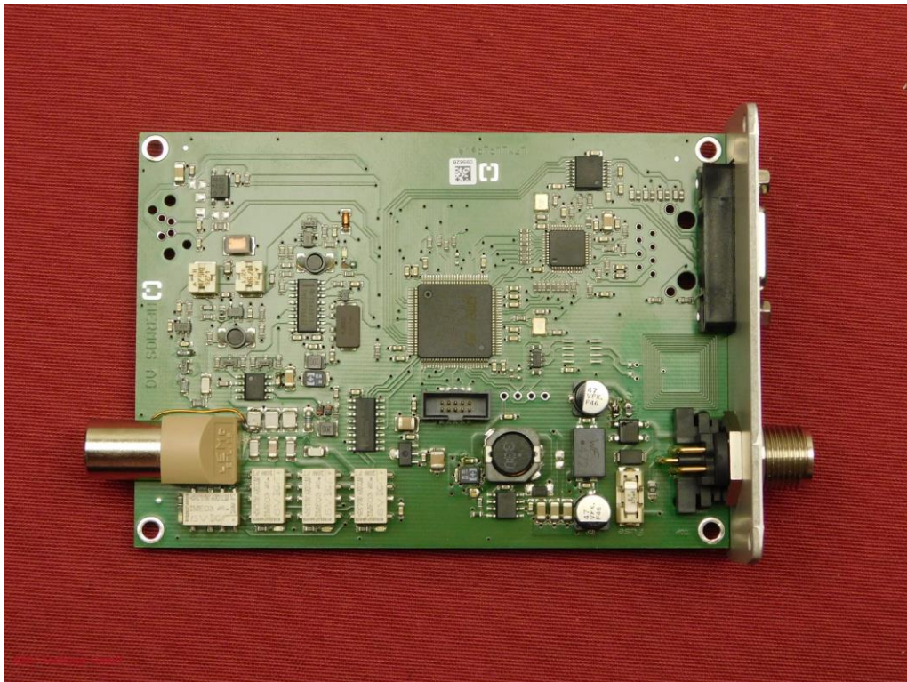
Picture 5: PCB - top side, without any housing
