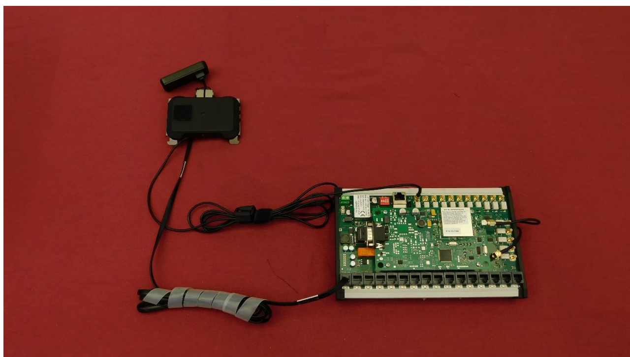
Picture 3: EUT – top view without housing
