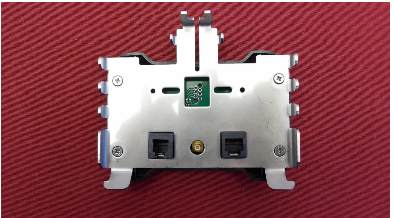
Picture 9: Antenna of EUT - bottom view
