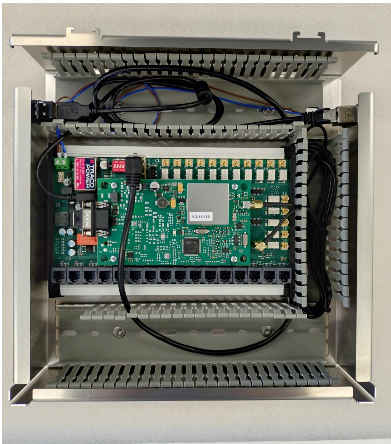
Picture 1: EUT – top view with housing
