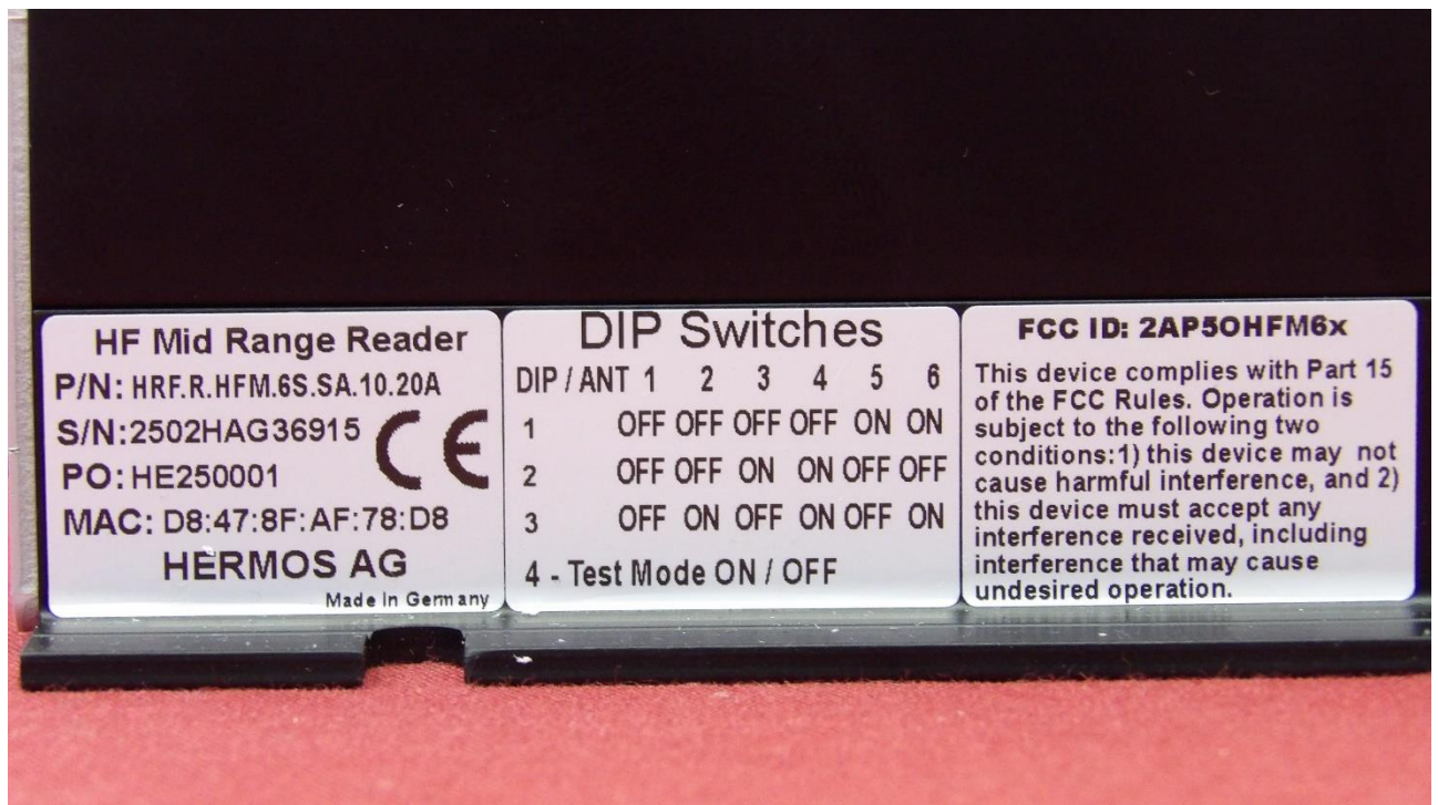
Picture 9: Preliminary name plate of EUT (not final version of the label)
