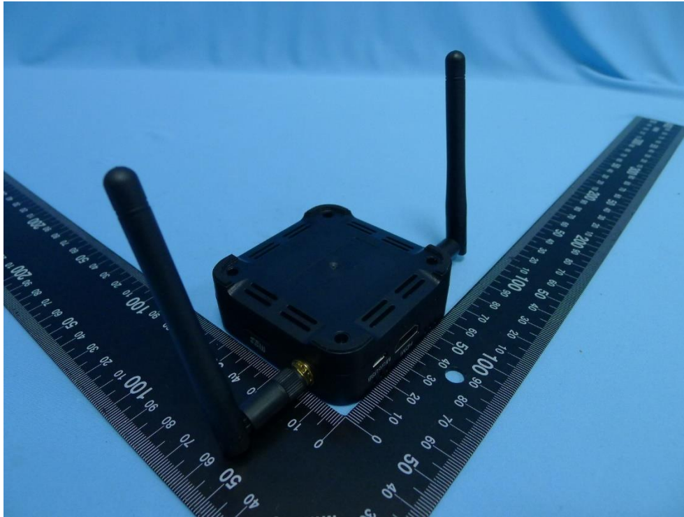
(8) EUT Photo- CT1200 (External Antenna)
