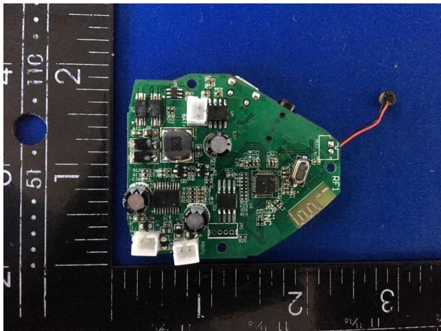
Mainboard-Rear View
