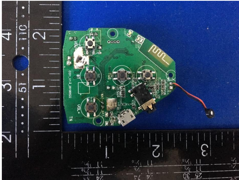
Mainboard-Front View
