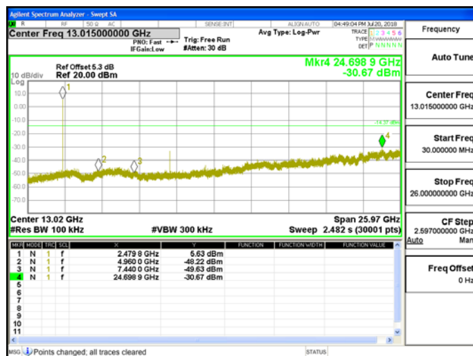
Spurious Emission_π/4DQPSK_2M_2480MHz
