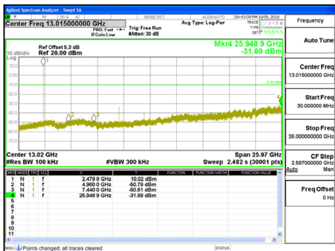
Spurious Emission_GFSK_1M_DH5_2480MHz
