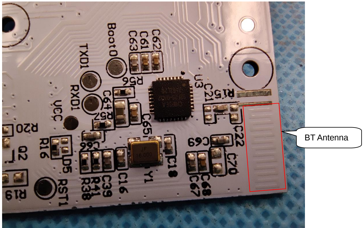
INTERNAL VIEW OF EUT (FIGURE 6)
