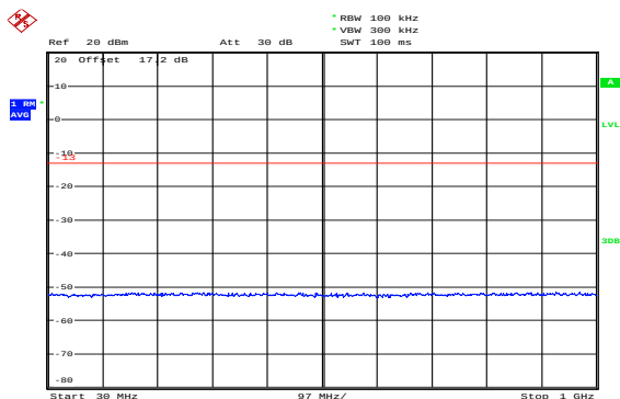
NB-IOT Band 4 3.75KHz 1@0 CH-Middle 30MHz~1GHz
