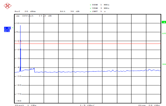
NB-IOT Band 4 3.75KHz 1@0 CH-Middle 1GHz ~20GHz
