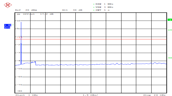
NB-IOT Band 4 3.75KHz 1@0 CH- High 1GHz ~20GHz
