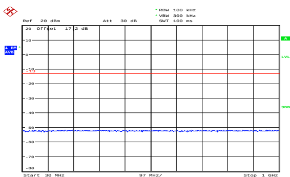
NB-IOT Band 4 3.75KHz 1@0 CH- High 30MHz~1GHz
