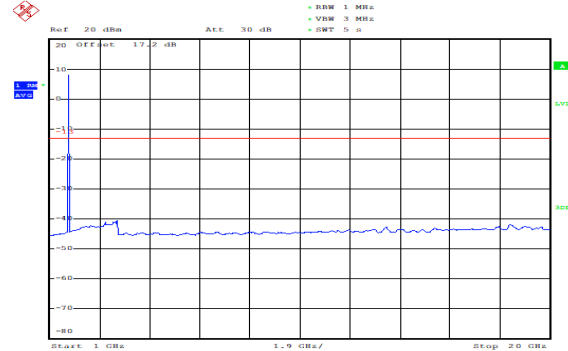
NB-IOT Band 4 3.75KHz 1@0 CH-Low 1GHz ~20GHz
