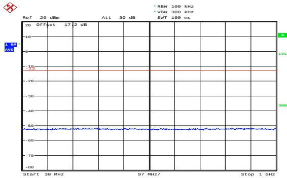
NB-IOT Band 4 3.75KHz 1@0 CH-Low 30MHz~1GHz
