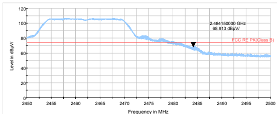
802.11g-Channel 11 Peak
