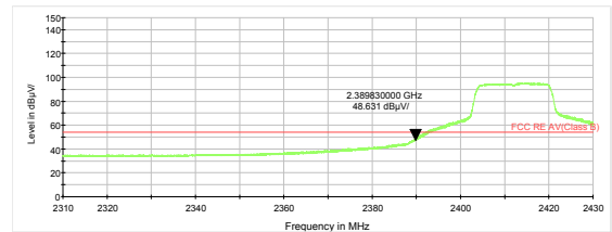
802.11g-Channel 1 Average
