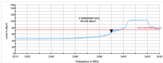
802.11g-Channel 1 Peak
