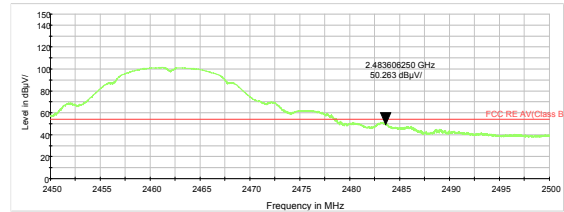
802.11b-Channel 11 Average
