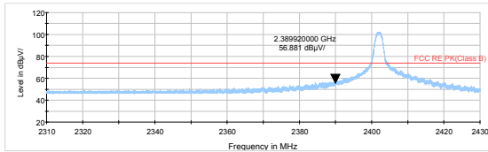
BLE Channel 0 Peak
