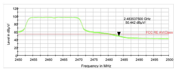
802.11g-Channel 11 Average
