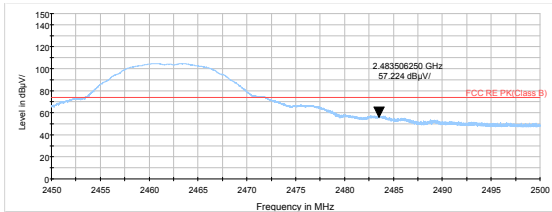
802.11b-Channel 11 Peak
