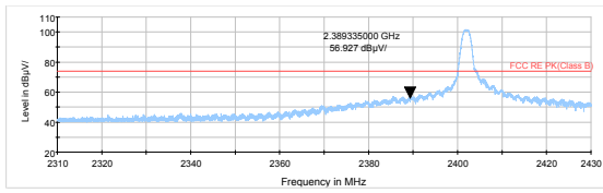
BLE Channel 0 Peak
