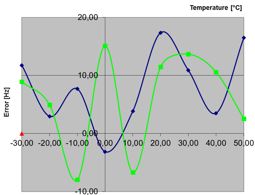
Frequency Error due to temperature variations
