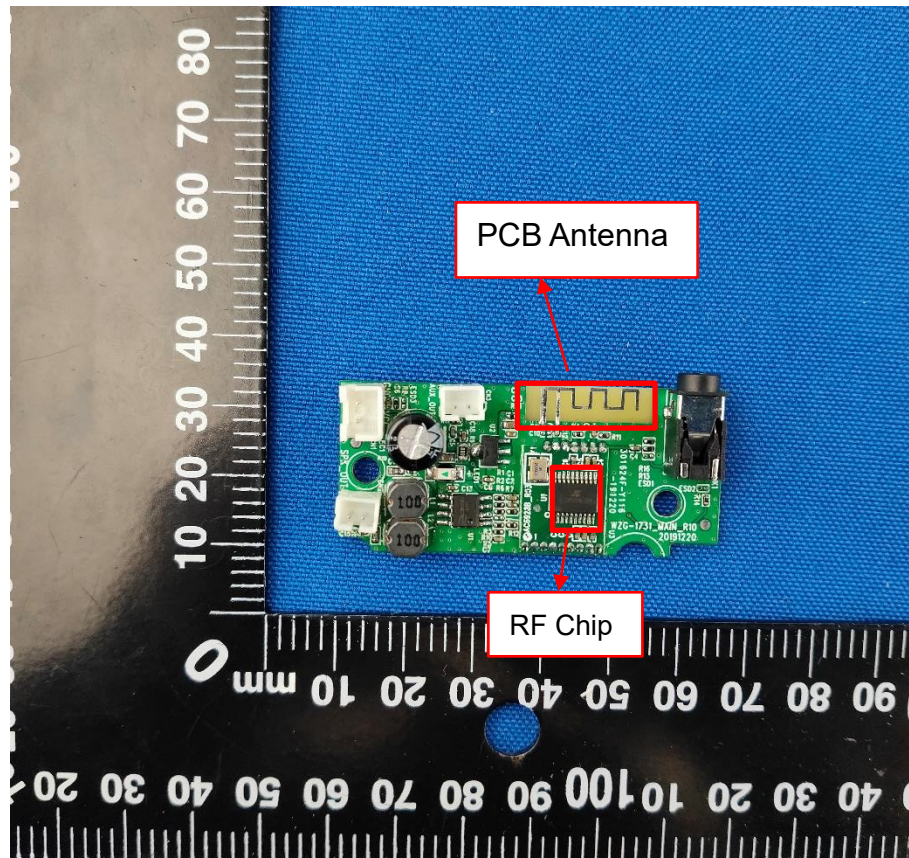
MAIN BOARD TOP VIEW
