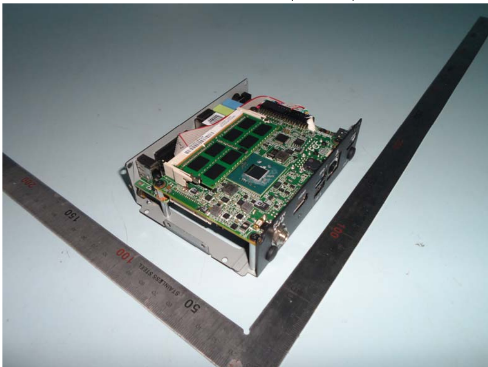
Inside View of The Product(Controller)
