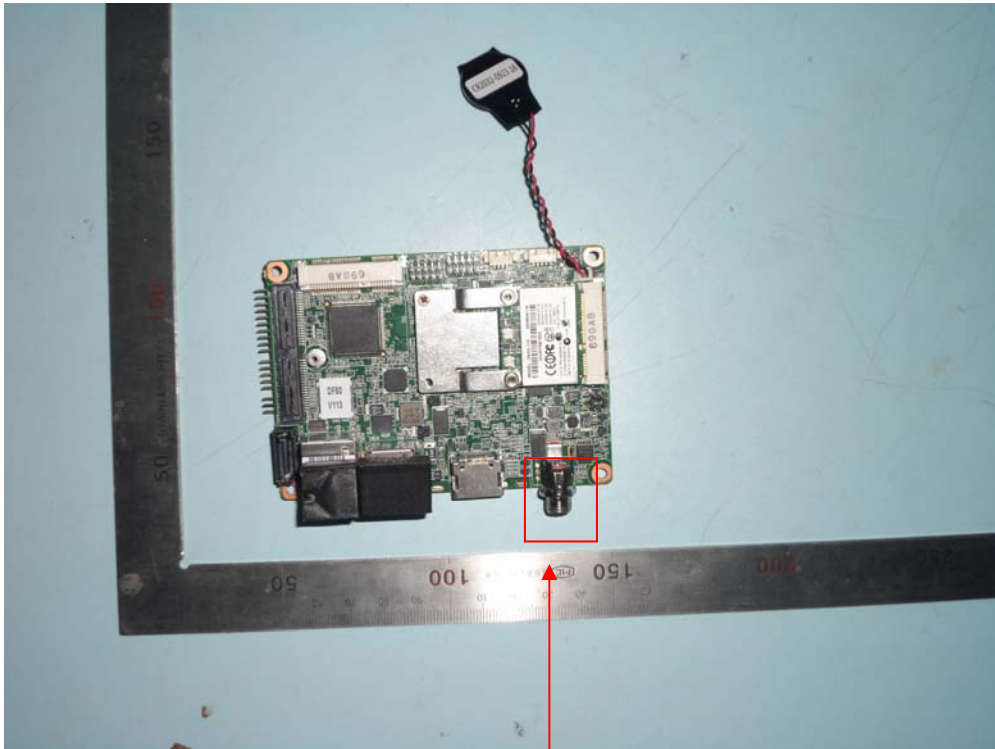
Inner Circuit Top View(Controller)
