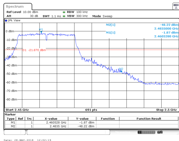
802.11g: Band Edge-High Channel
