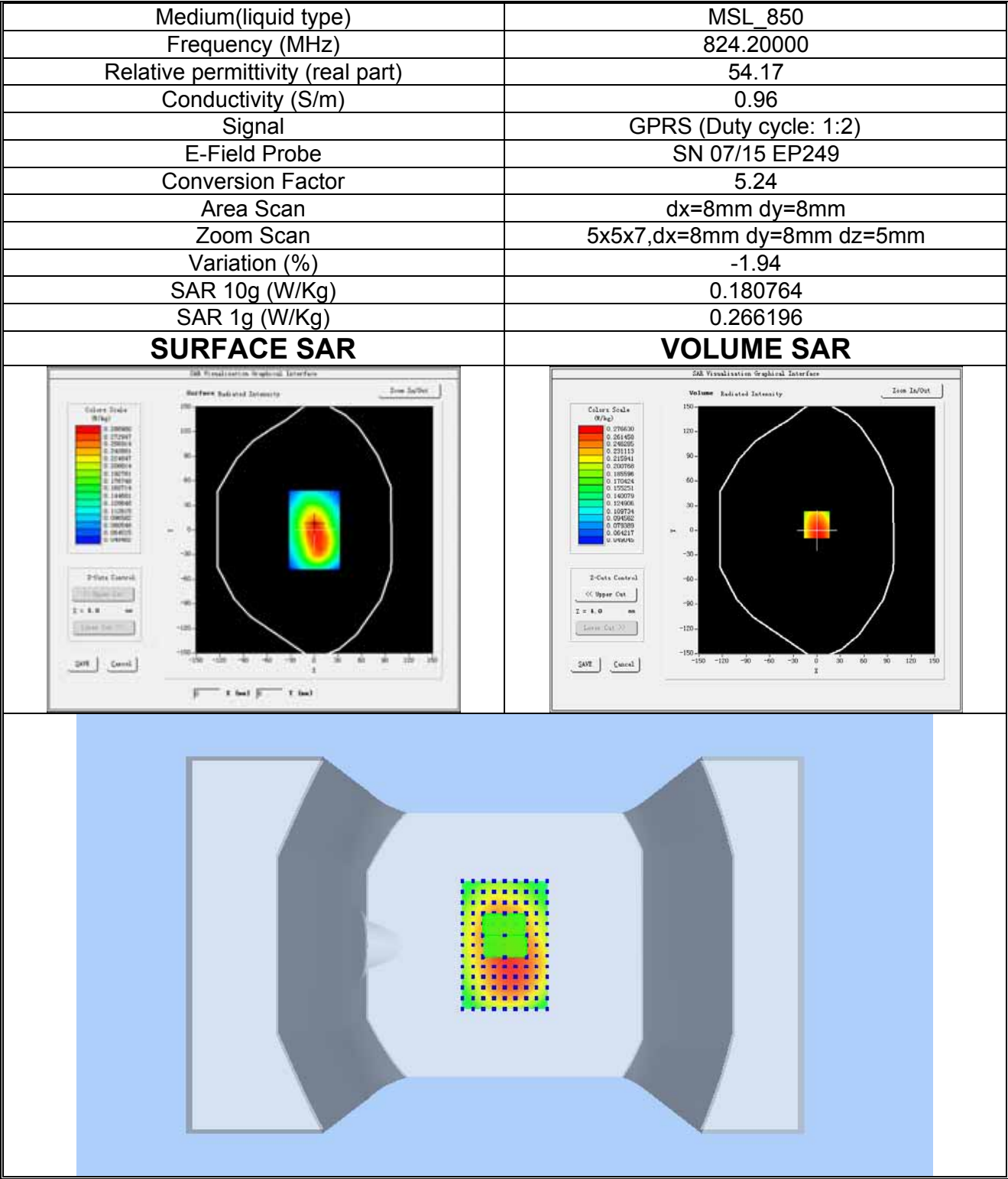
Plot 7: GPRS850MHz, Low channel(Body-worn, Right edge) Product Description: Mobile Phone Test Date: 2018-06-07
