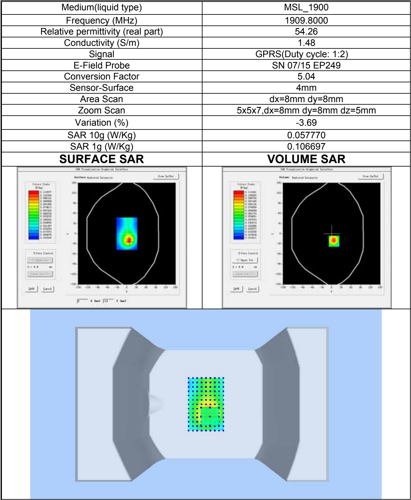
Plot 15: GPRS1900, High channel(Body-worn,Right edge) Product Description: Mobile Phone Test Date: 2018-06-08
