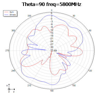
Theta=90 freq=5800MHz
