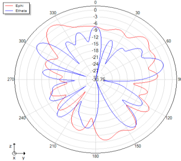
Phi=90 freq=5500MHz
