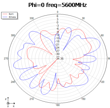
Phi=0 freq=5600MHz
