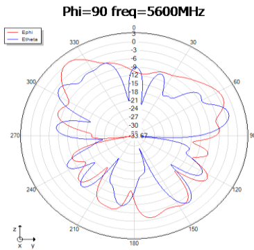
Phi=90 freq=5600MHz
