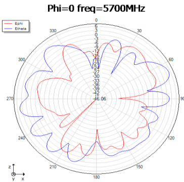
Phi=0 freq=5700MHz
