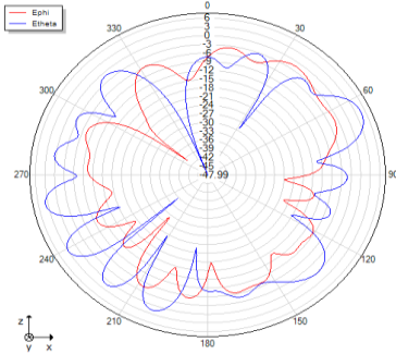
Phi=0 freq=5500MHz
