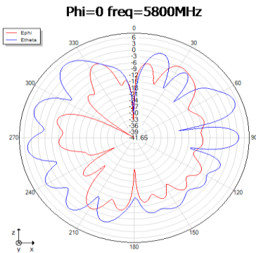
Phi=0 freq=5800MHz
