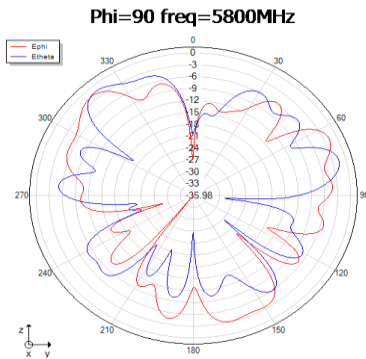
Phi=90 freq=5800MHz
