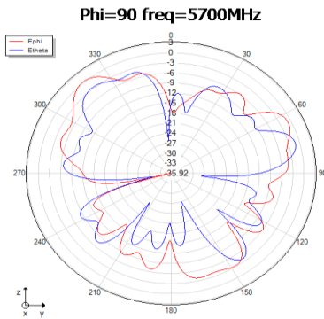
Phi=90 freq=5700MHz
