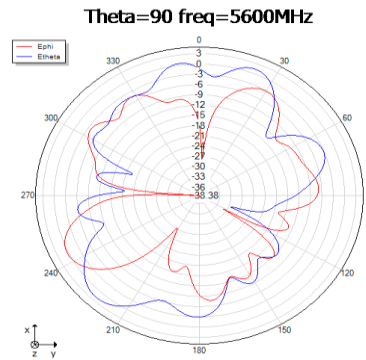
Theta=90 freq=5600MHz
