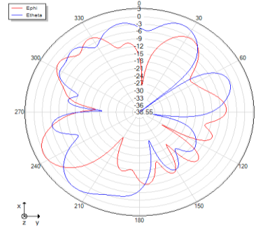
Theta=90 freq=5500MHz
