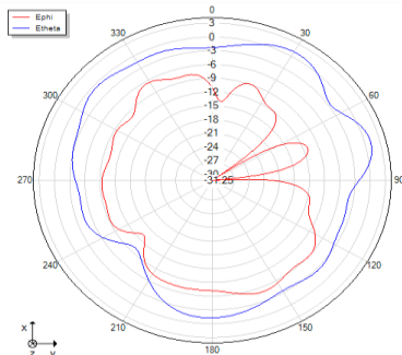
Theta=90 freq=2430MHz
