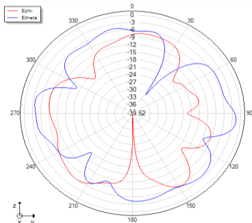
Phi=90 freq=2430MHz
