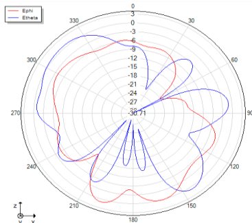
Phi=0 freq=2430MHz
