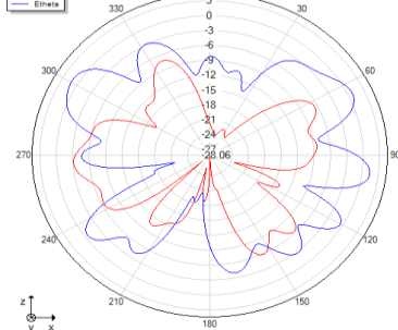
Phi=0 freq=5700MHz
