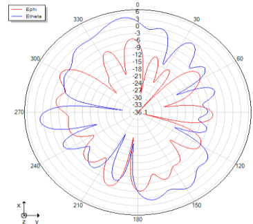
Theta=90 freq=5800MHz
