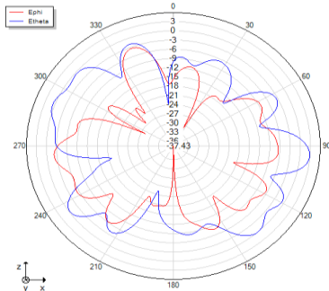
Phi=0 freq=5800MHz
