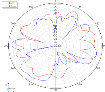
Phi=90 freq=5700MHz
