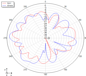
Phi=90 freq=5800MHz
