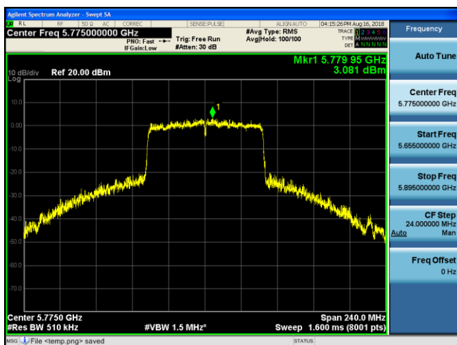
Channel 155 / 5775 MHz
