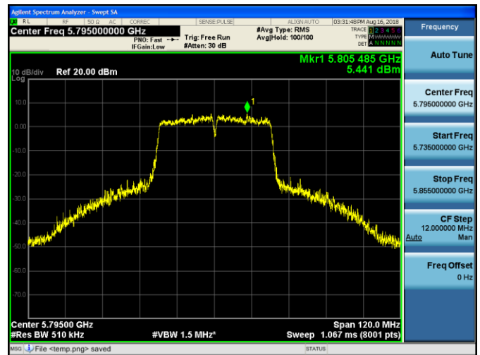
Channel 159 / 5795 MHz
