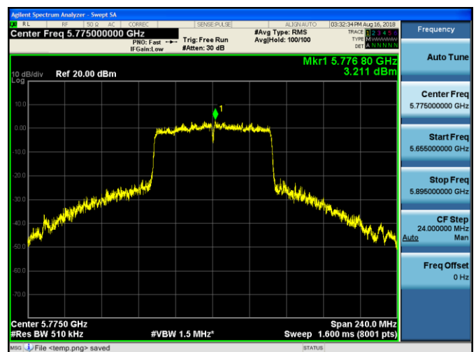
Channel 155 / 5775 MHz
