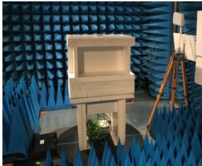
General Test setup in anechoic chamber >1GHz
