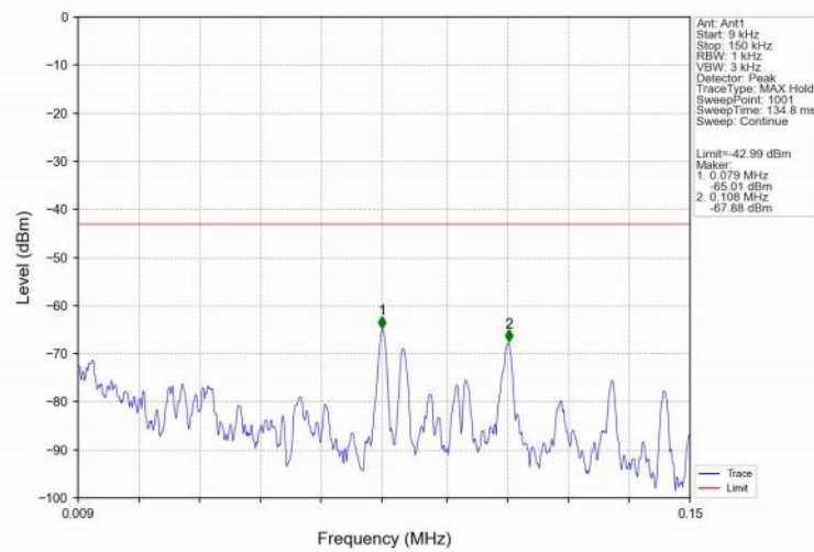
8DPSK_3DH5_LCH_2402MHz_Ant1_NTNV
