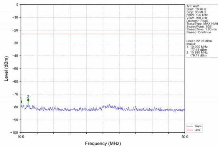
GFSK_DH5_MCH_2441MHz_Ant1_NTNV
