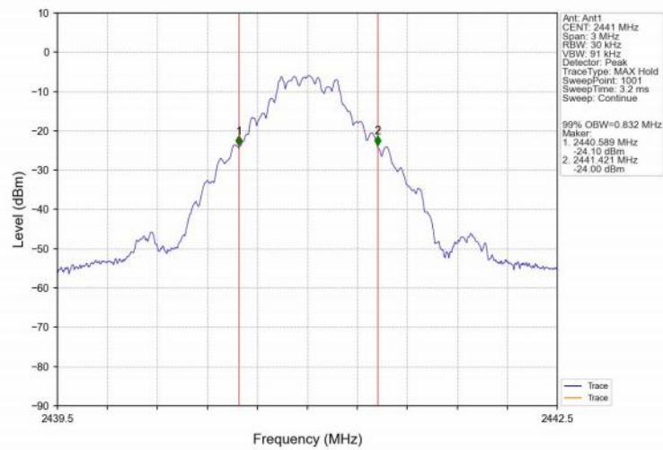
GFSK_DH5_MCH_2441MHz_Ant1_NTNV
