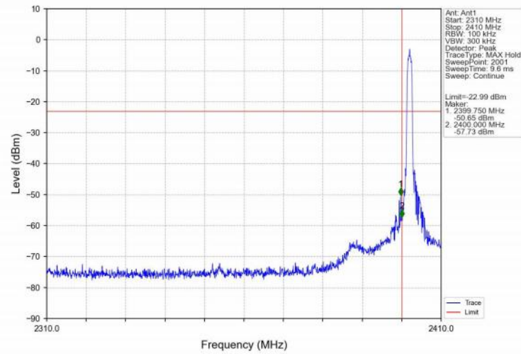
8DPSK_3DH5_LCH_2402MHz_Ant1_NTNV
