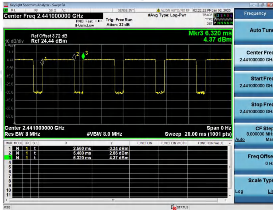
Duty_Cycle_NVNT_ANT1_3-DH5_2441
