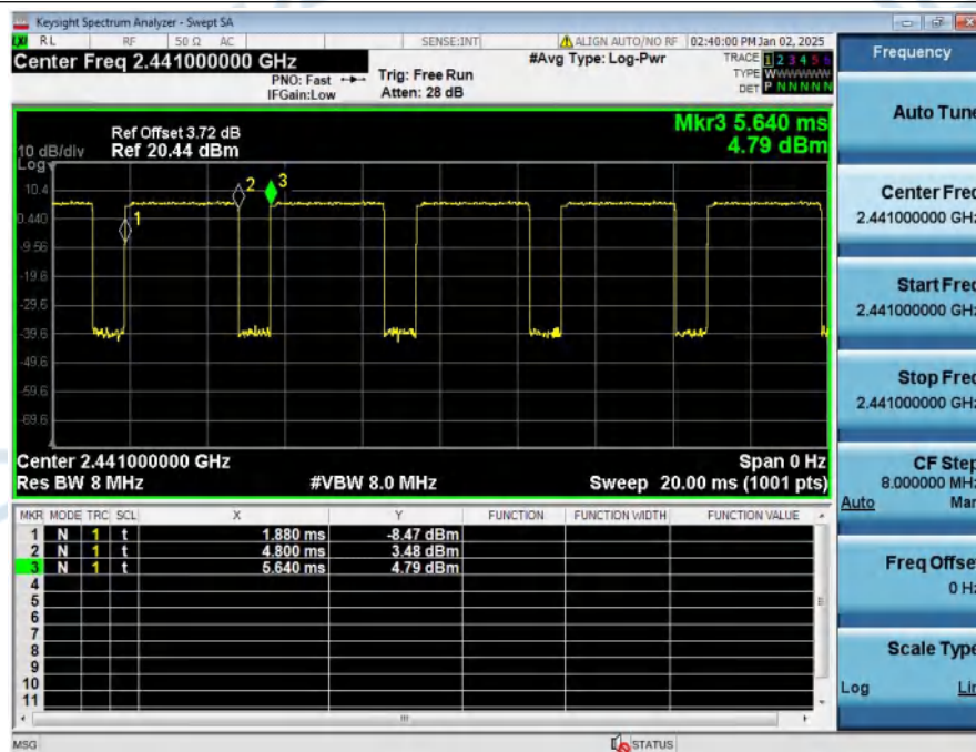
Duty_Cycle_NVNT_ANT1_3-DH5_2441
