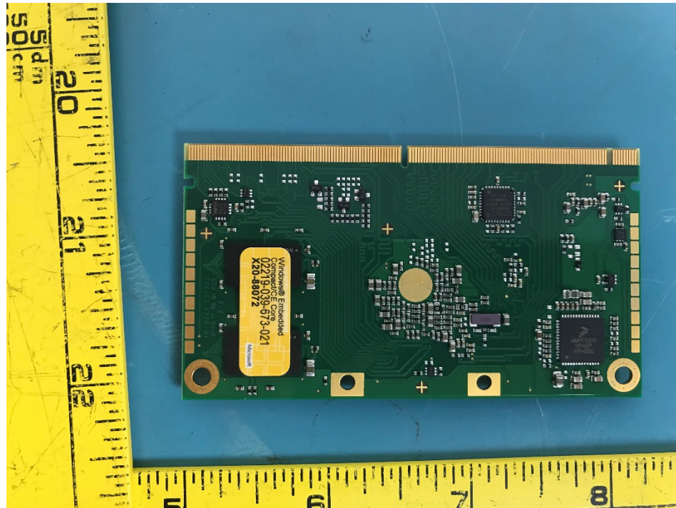
EUT Board 2 Bottom View
