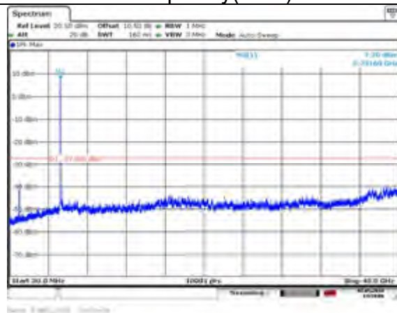
802.11n HT40 (SISO Ant0) Carrier frequency(MHz):5230
