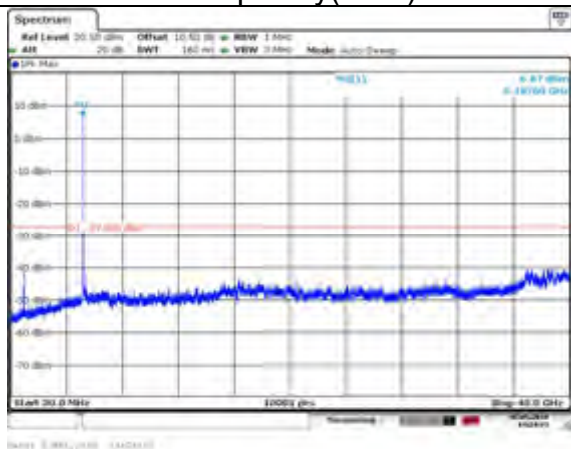
802.11n HT40 (MIMO Ant0) Carrier frequency(MHz):5190
