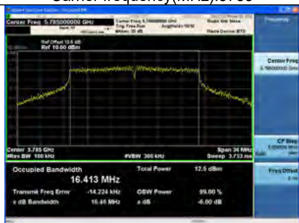
802.11a Carrier frequency(MHz):5785
