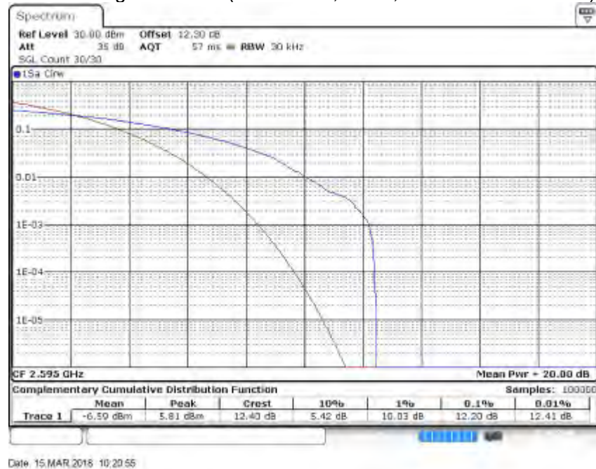
Peak-Average Ratio Plot(15MHz BW,16QAM,Band 41-mid Channel)
