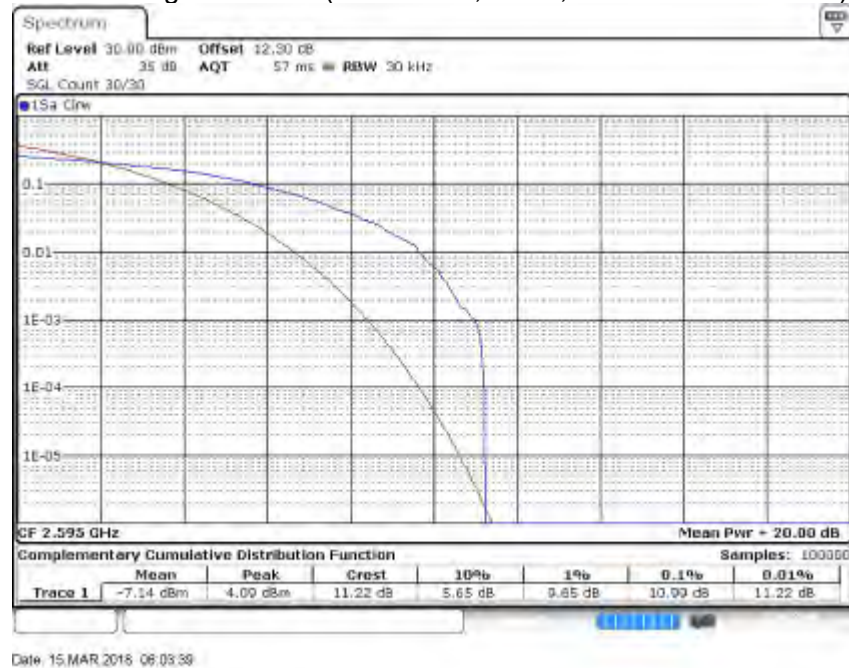
Peak-Average Ratio Plot(20MHz BW,16QAM,Band 38-mid Channel)
