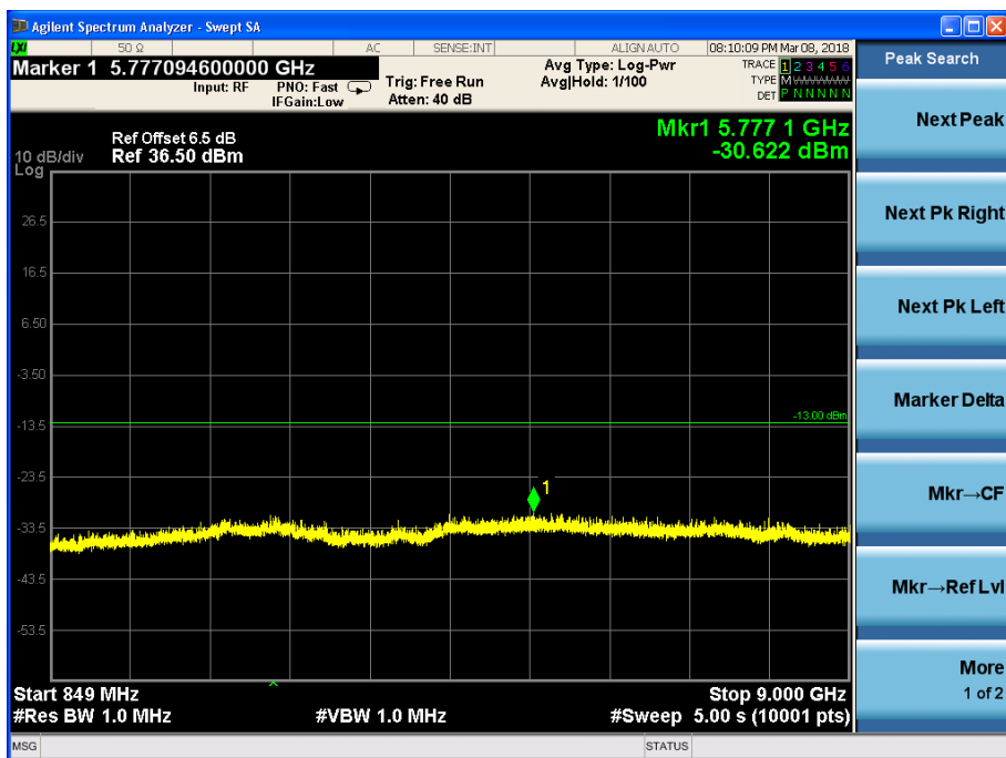
Channel 189, 849MHz~9GHz
