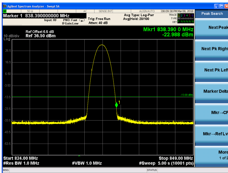
Channel 189, 824MHz~849MHz
