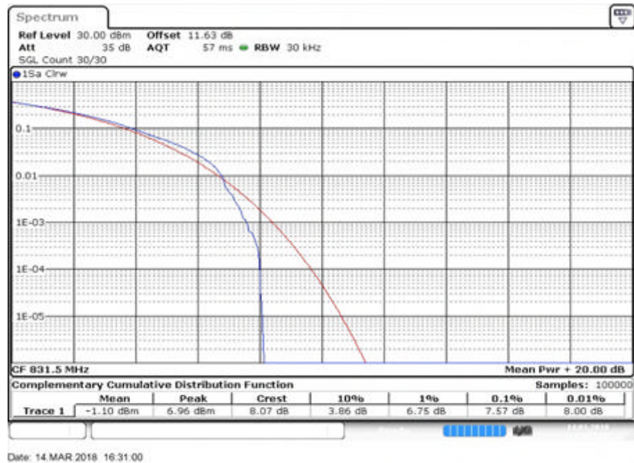
Peak-Average Ratio Plot(15MHz BW,QPSK,Band 26-mid Channel)
