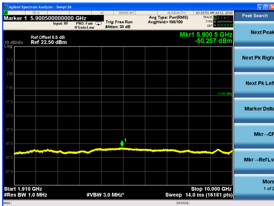
Channel 600, 1910MHz~10GHz
