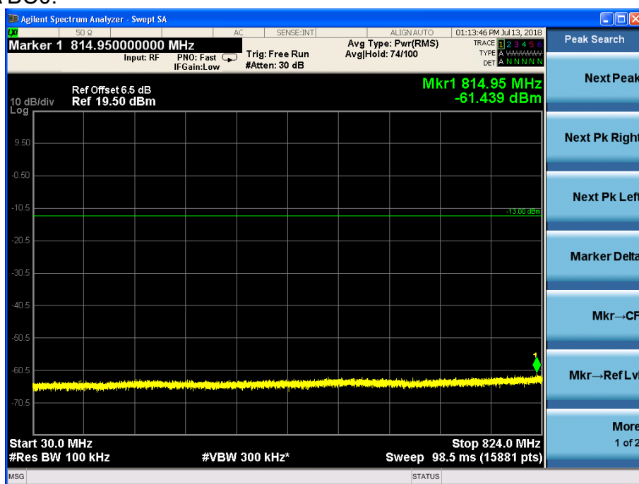
Channel 384, 30MHz~824MHz
