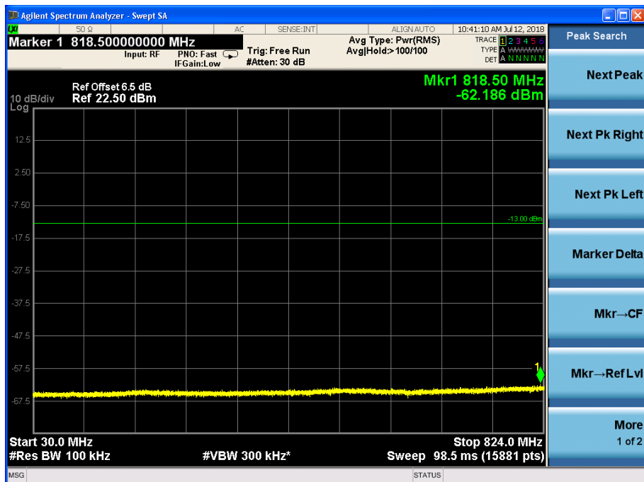
Channel 384, 30MHz~824MHz
