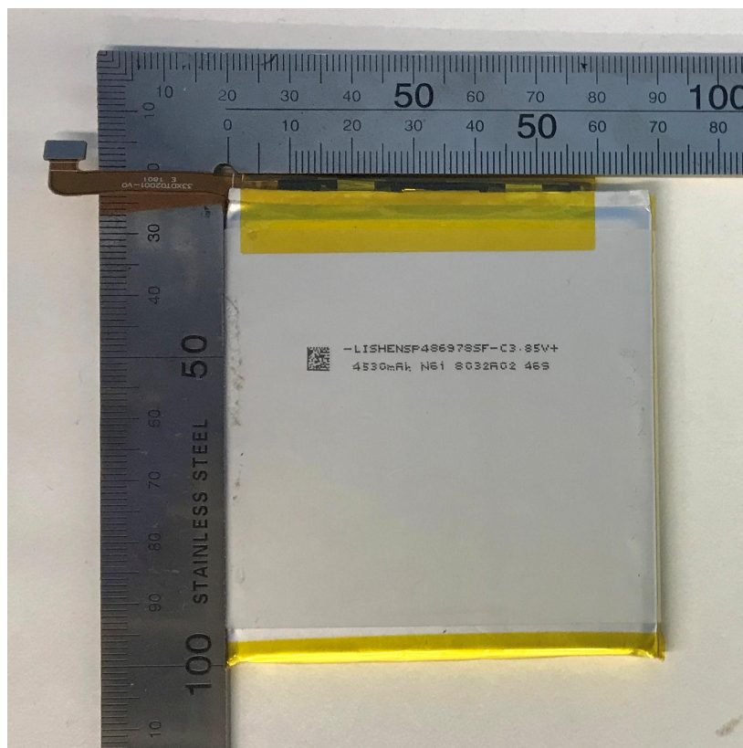
Battery (FJ-SW1260502000DN Made by SHENZHEN FUJIA APPLIANCE CO., LTD.)
