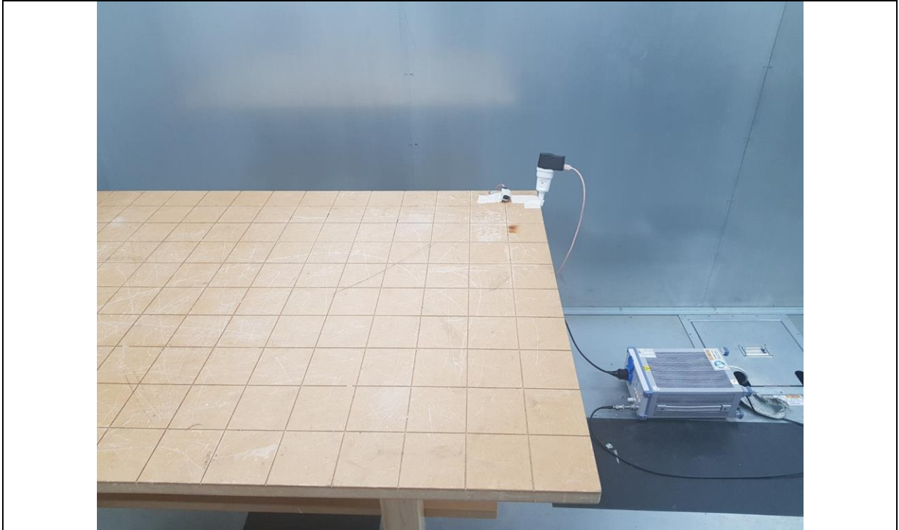
Conducted Emission_Front
