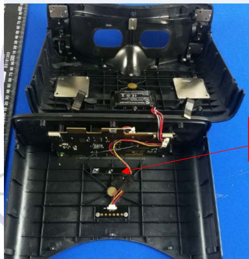
WiFi/BT Antenna
