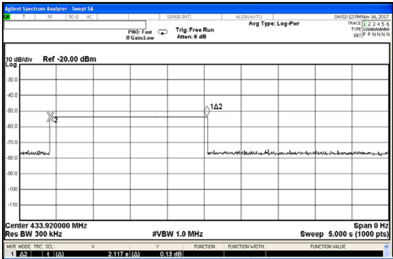
Plot 7.1.1 Transmitter shut down test result (operated manually and activated automatically)
