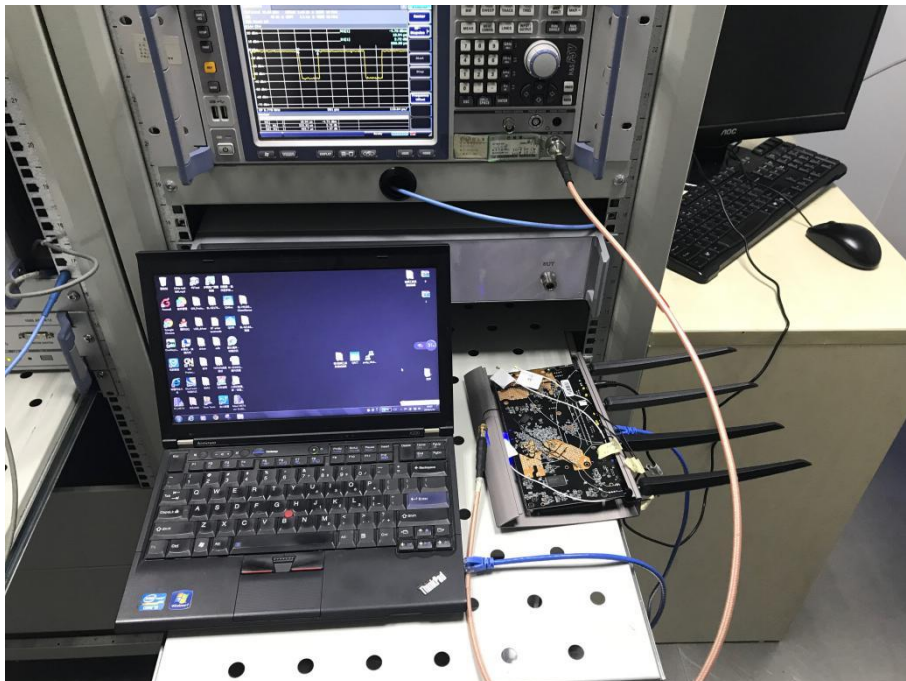
Conducted Test 1
