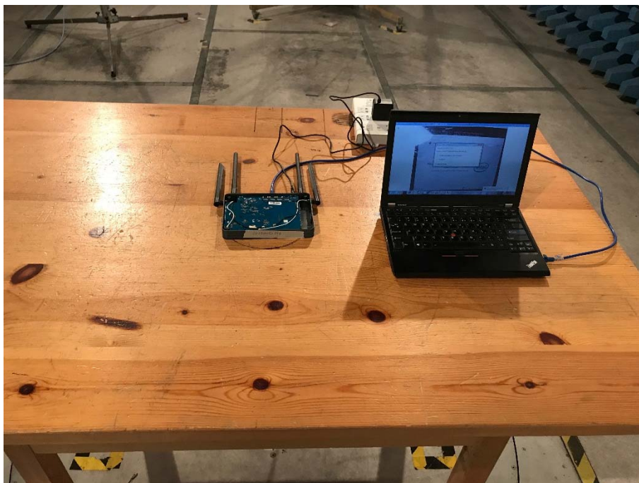
30 MHz-1 GHz (RSE)
