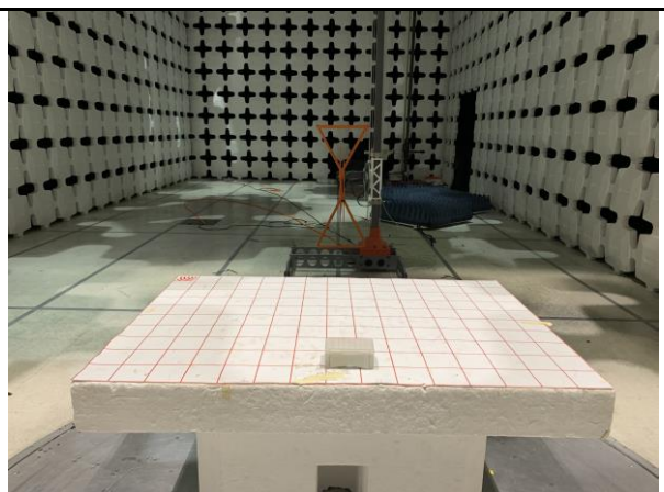
Radiated Emission Test below 1GHz Rear View
