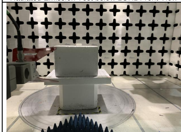
Radiated Emission Test above 1GHz Front View
