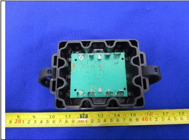
EUT-PCB Top View
