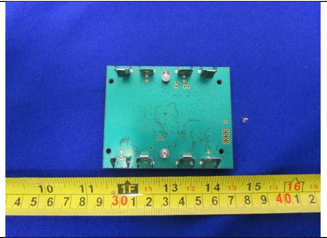
EUT-PCB- Top View 2
