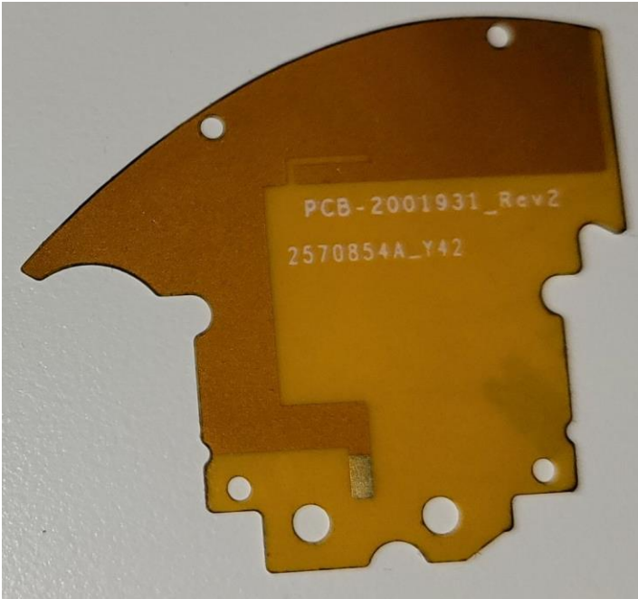
Dual Band ISM Antenna (902-928MHz & 2400-2483.5MHz) PCB top
