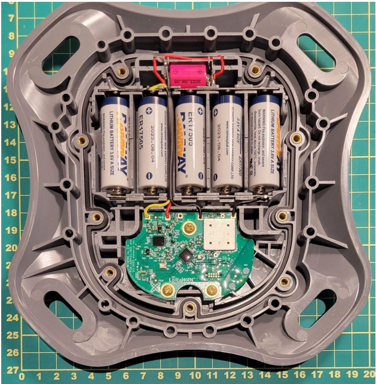
PCB with battery in enclosure top
