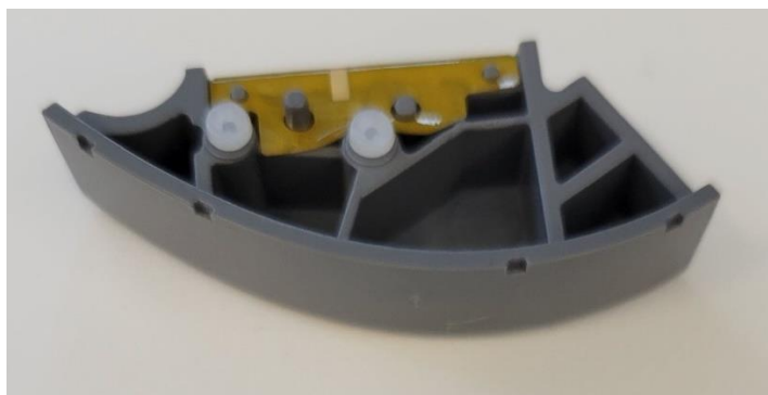
Dual Band ISM Antenna (902-928MHz & 2400-2483.5MHz) Assembly Bottom
