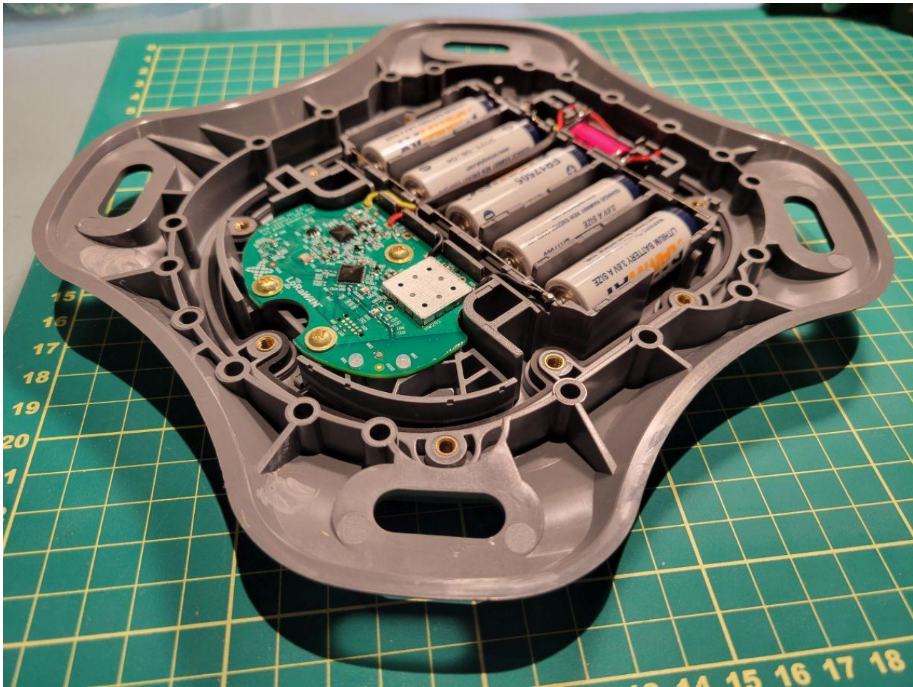
PCB with battery in enclosure side
