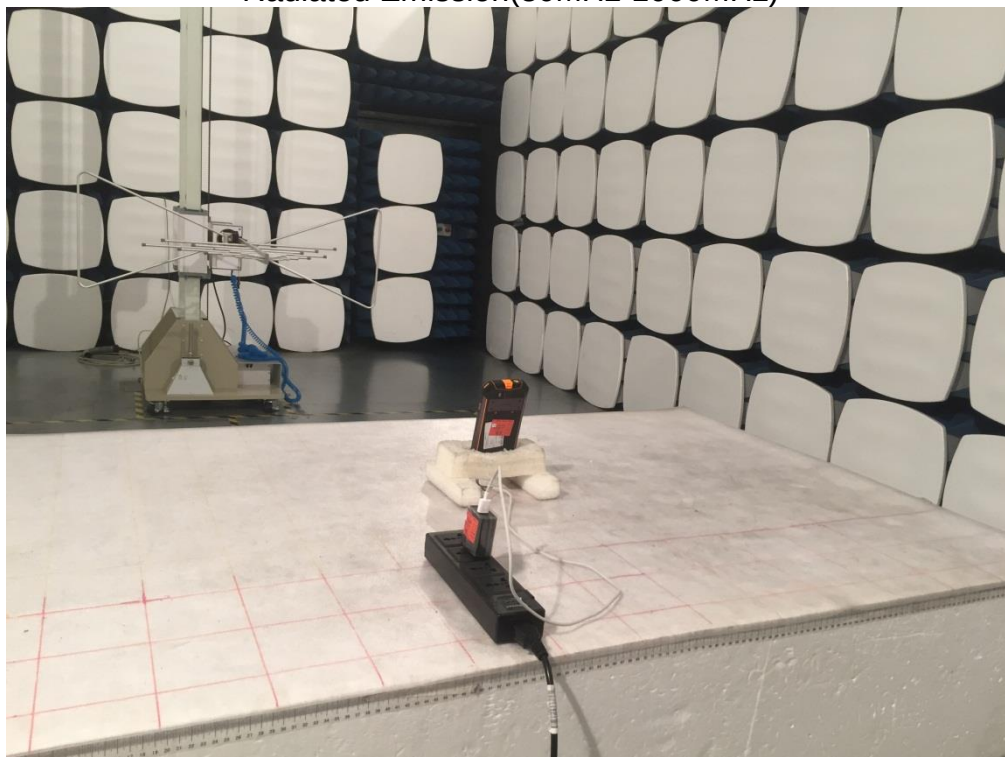
Radiated Emission(30MHz-1000MHz)
