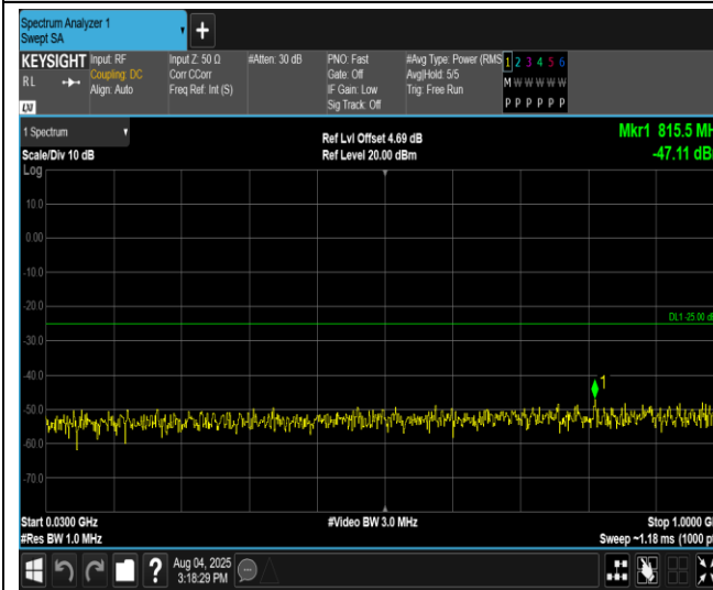
Band41-5MHz-64QAM-39675-1RB#0-Range1:30~1000MHz
