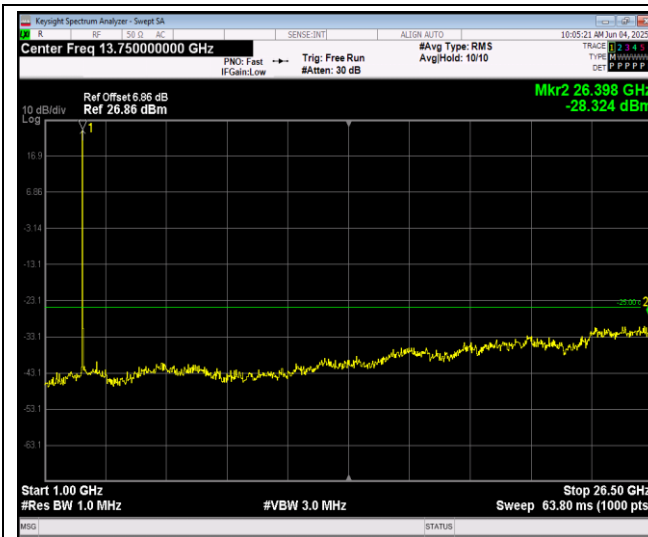
Band41-5MHz-16QAM-41565-1RB#0-Range2:1000~26500MHz
