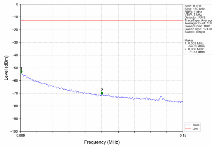
Band4_HSDPA_MCH_1732.6MHz_Subtest 1_NTNV
