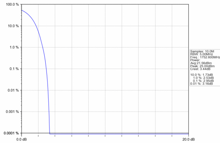
Band4_RMC_HCH_1752.6MHz_12.2kbps RMC_NTNV
