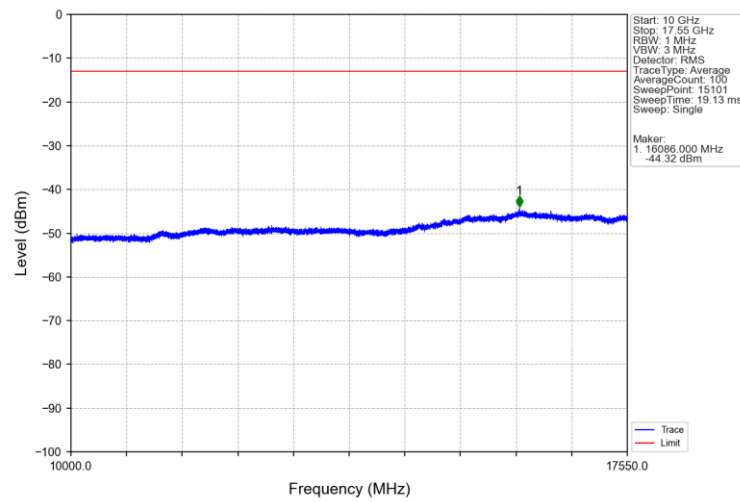
Band4_RMC_LCH_1712.4MHz_12.2kbps RMC_NTNV
