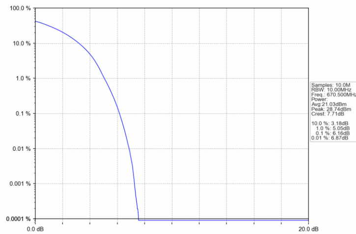
Band71_15MHz_16QAM_LCH_670.5MHz_RB_75_0_NTNV
