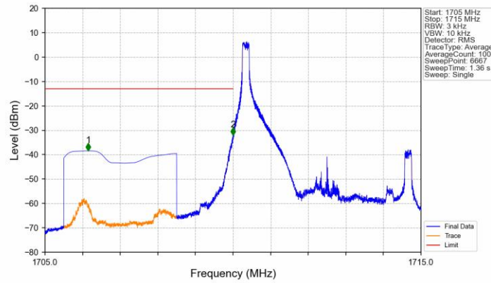
Band4_5MHz_QPSK_LCH_1712.5MHz_RB_1_0_NTNV
