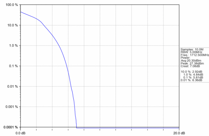
Band4_5MHz_16QAM_LCH_1712.5MHz_RB_25_0_NTNV
