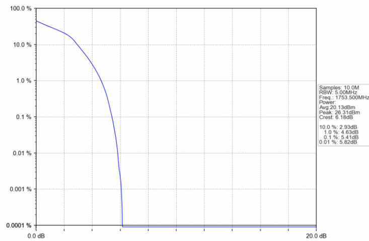
Band4_3MHz_16QAM_HCH_1753.5MHz_RB_15_0_NTNV
