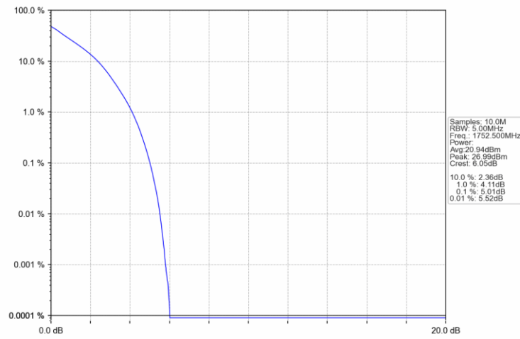
Band4_5MHz_QPSK_HCH_1752.5MHz_RB_25_0_NTNV
