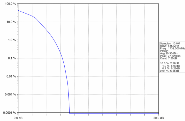
Band4_3MHz_16QAM_MCH_1732.5MHz_RB_15_0_NTNV
